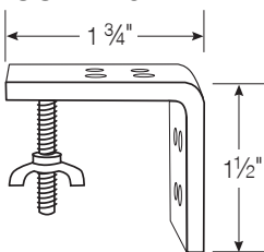
Mounting Bracket and Screws (clutch and cordless shades)
